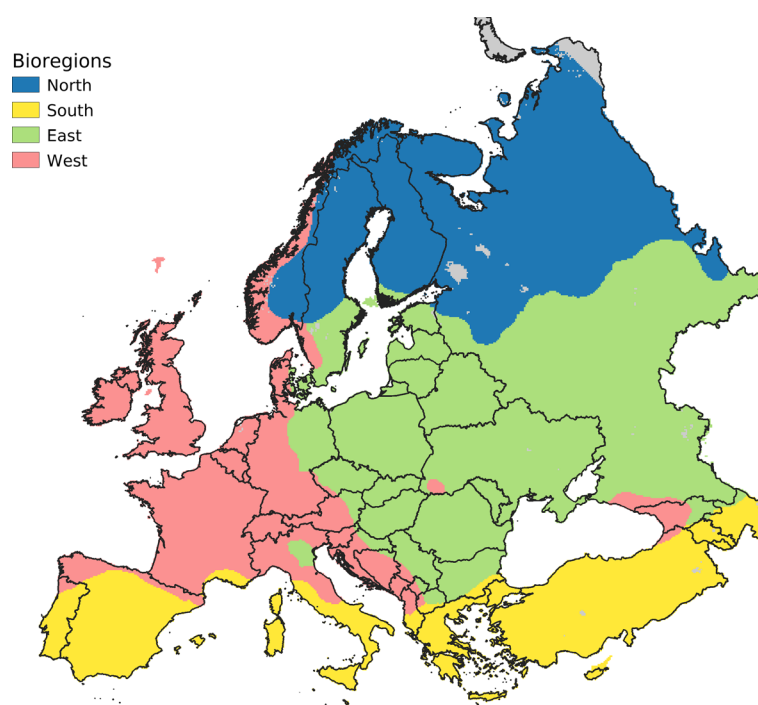
Figure 1: Homogeneous bioclimatic regions (Bioregions) of Europe based on bioclimatic variables, vegetation cover and topographic covariates associated to wild boar density (Source: ENETWILD Consortium et al., 2019a,b, 2020a)
